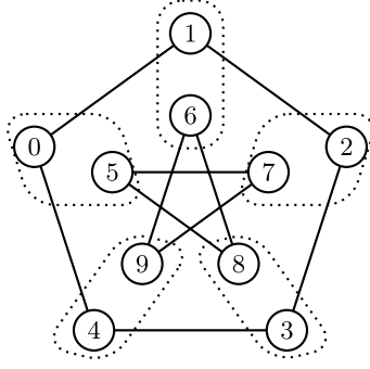
Fig. 1. Partitioned graph and its partition line-graph.
