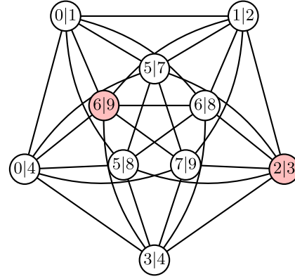
Fig. 1. Partitioned graph and its partition line-graph.
