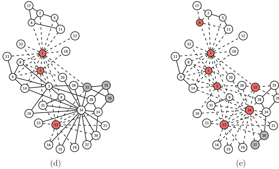
Fig. 10. In part (d), we report an optimal CIP policy with k = 3 , depicting in red the interdicted vertices. In part (e), we report the same information for k = 7 . (For interpretation of the references to color in this figure legend, the reader is referred to the web version of this article.)
