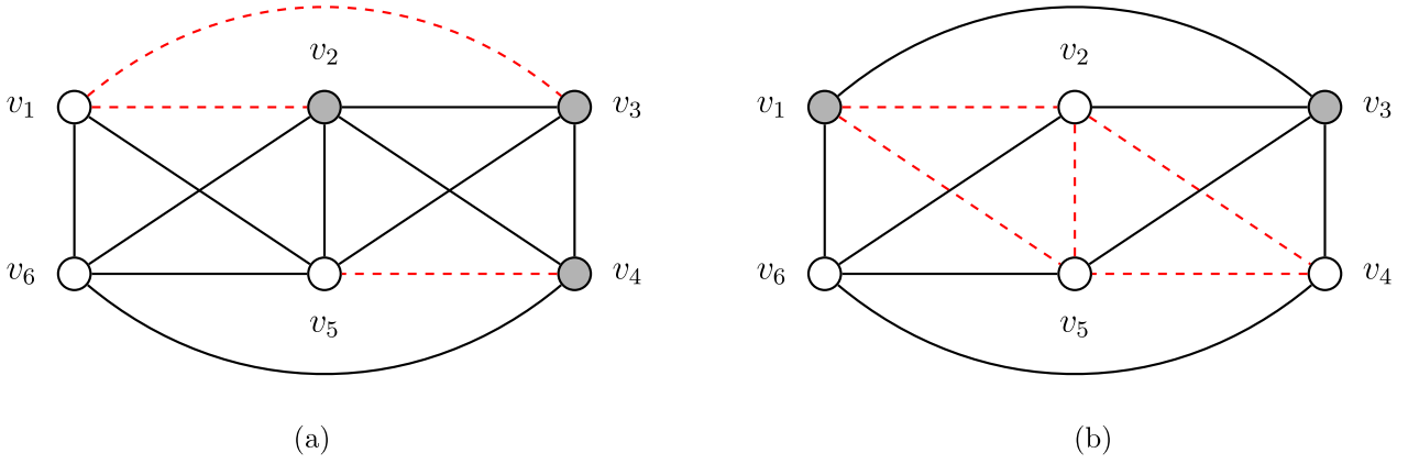
Fig. 2. Two optimal interdiction policies represented by dashed red edges with: (a) k = 3 and (b) k = 5 . With k = 3 , the interdicted graph G_I has \omega(G_I) = 3 and one of the largest cliques is \{v_2, v_3, v_4\} (grey vertices). With k = 5 , \omega(G_I) = 2 and one of the largest cliques is \{v_1, v_3\} (grey vertices). (For interpretation of the references to color in this figure legend, the reader is referred to the web version of this article.)
