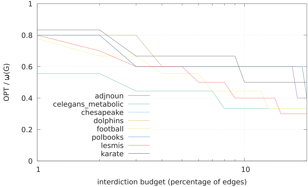
Fig. 8. The edge clique interdiction curves for 8 classical (social) networks from the 10th DIMACS challenge (DIMACS10, 2017).
