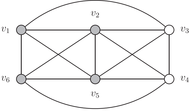
Fig. 1. An example graph G with 6 vertices and 13 edges. Before interdiction, the clique number is \omega(G) = 4 . One of the four maximum cliques is shown in grey, i.e., the clique \{v_1, v_2, v_5, v_6\} .
