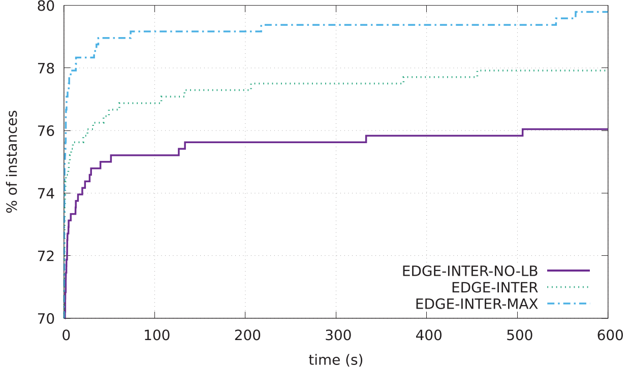
Fig. 7. Performance profile of the different configurations of EDGE-INTER for the DIMACS_2-Coloring graphs.
