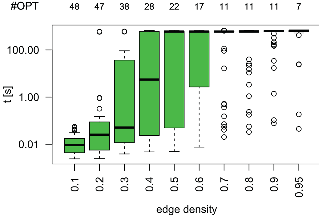
Fig. 6. Impact of the edge density on the computational performance of EDGE-INTER for the set of Erdős-Rényi graphs used for benchmarking.
