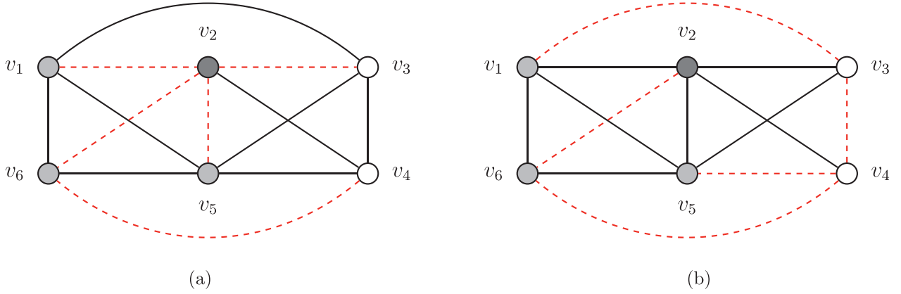
Fig. 5. Two different interdiction policies depicted in red dashed lines to show the effects of maximal cliques on the inequalities (5). (For interpretation of the references to color in this figure legend, the reader is referred to the web version of this article.)
