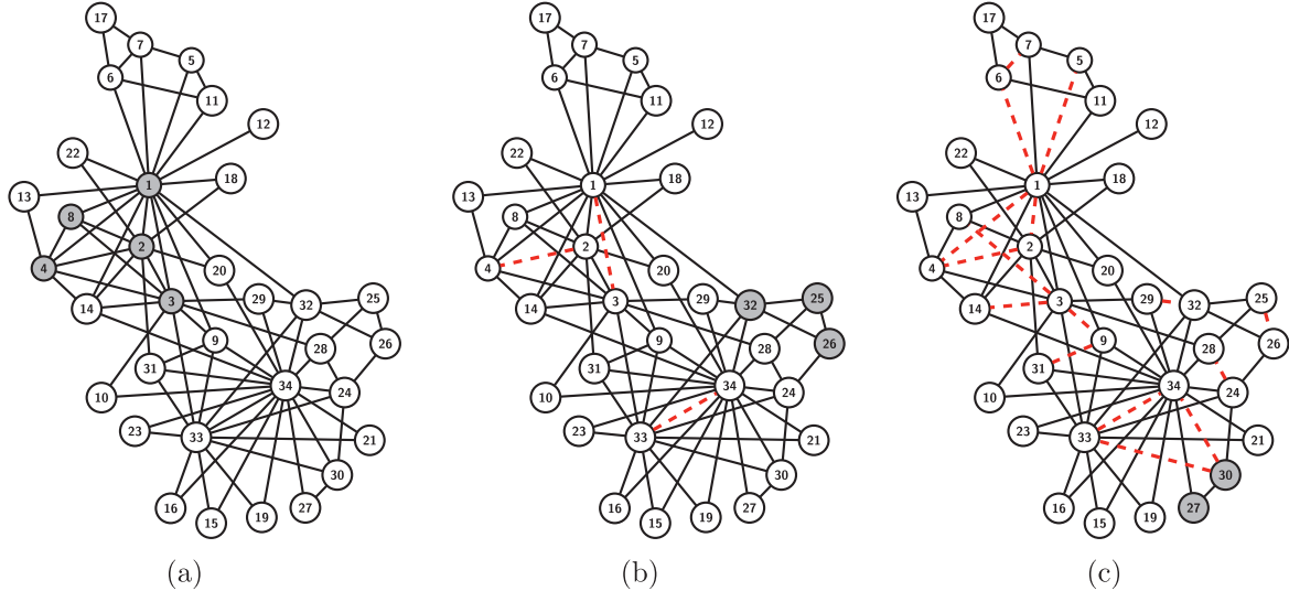
Fig. 9. In part (a), we report the karate social network, grey vertices correspond to a maximum clique of size 5. In part (b), we report an optimal EICP policy with k = 3 , depicting in dashed red the interdicted edges. In this case, the size of the maximum clique in the interdicted graph is 3 and the grey vertices correspond to a maximum clique. In part (c), we report the same information for k = 16 . (For interpretation of the references to color in this figure legend, the reader is referred to the web version of this article.)
