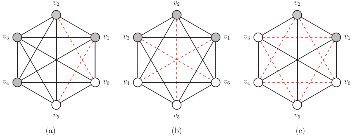
Fig. 3. An example clique of size 6. The minimum number of edges to remove from the clique to reduce the clique size to 4 is 2, to 3 is 3 and to 2 is 6. (For interpretation of the references to color in this figure, the reader is referred to the web version of this article.)
