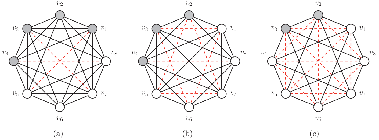
Fig. 4. An example clique of size 8. The minimum number of edges to remove from the clique to reduce the clique size to 4 is 4, to 3 is 7 and to 2 is 12. (For interpretation of the references to color in this figure, the reader is referred to the web version of this article.)
