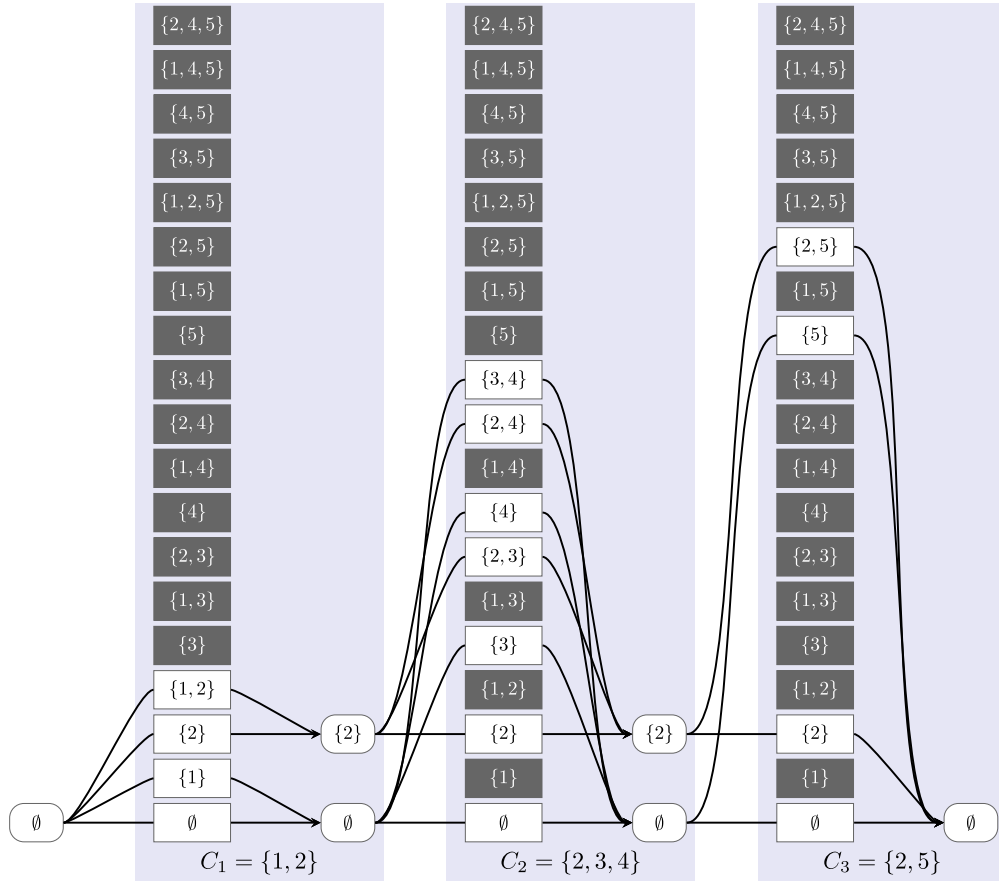
Fig. 3. The combinatorial arcflow graph for E_0 consisting of four layers, six nodes, and 15 arcs. In contrast to the idea presented in Caprara et al. (2013) , the arc and node labels carry some information relevant to the respective clique (so that, in our visualization, both of them are related to the blue background indicating a specific maximal clique). For the sake of completeness and to better understand the overall construction process, we depicted the entire pattern set \mathcal{P} in any layer, but cancelled out the elements that are infeasible because they do not use the items allowed for the respective clique. Those infeasible subpatterns are colored black and do not belong to any arc. (For interpretation of the references to colour in this figure legend, the reader is referred to the web version of this article.)
