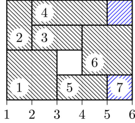
Fig. 2. An assignment of seven items to one bin of size C=5 , following an idea from bandwidth allocation in wireless networks, see Chen et al. (2002) . The blue item i=7 with [s_i, e_i] = [5, 6] and c_i=2 is not placed in a connected manner. Moreover, there is no rearrangement of the items that enables representing item i=7 as a single rectangle of size 1 \times 2 , without destroying the rectangular structure of another item. In particular, this packing would not be feasible for the strip packing problem (SPP). (For interpretation of the references to colour in this figure legend, the reader is referred to the web version of this article.)
