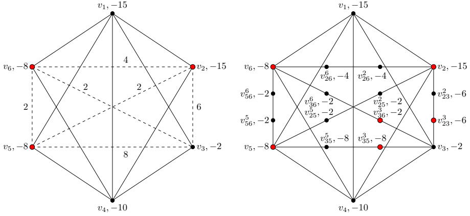
Fig. 1 Example: a graph G (left) and the corresponding extended graph \tilde{G} (right)
