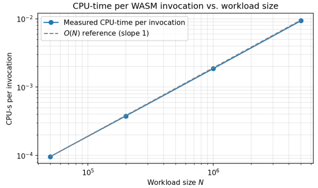
Figure 11: Measured CPU-time per WASM invocation vs. workload size N (log-log; cgroup cpu.stat , exact), against an O(N) reference line of slope 1.
