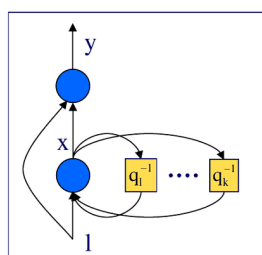
Graphical model for trees
