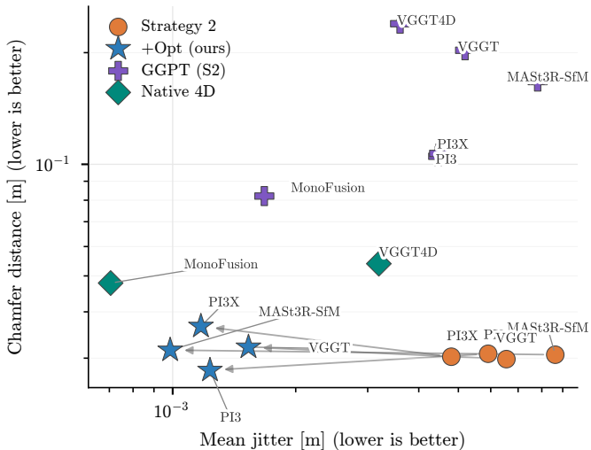
Geometry vs. temporal consistency (DexYCB, pooled over views)
