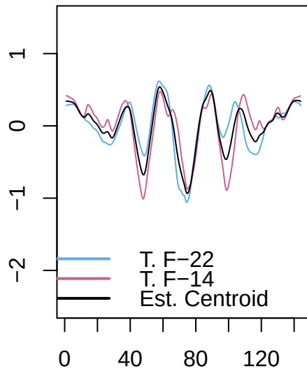
Centroids
