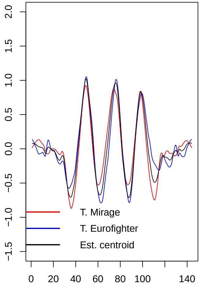
Centroids
