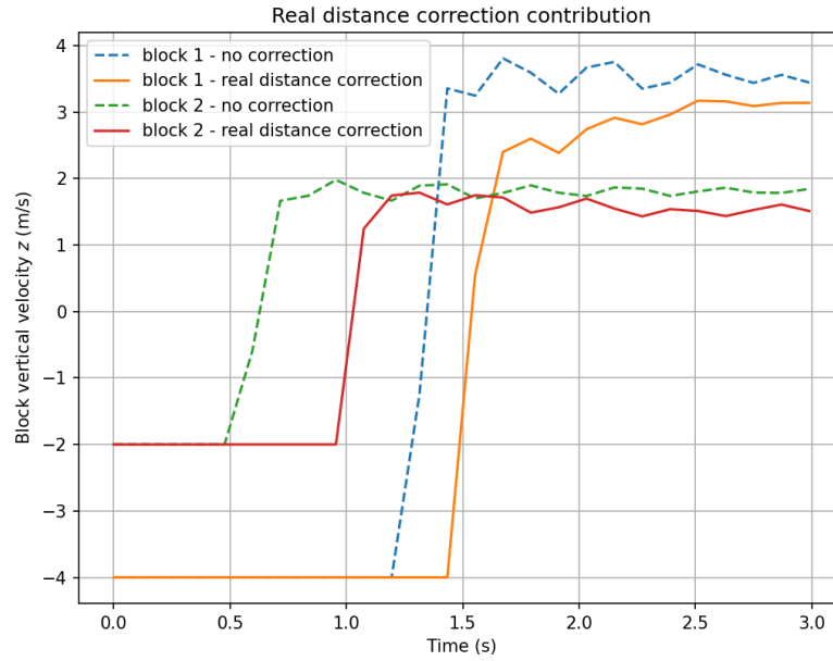
Figure 6: Velocity comparison.
