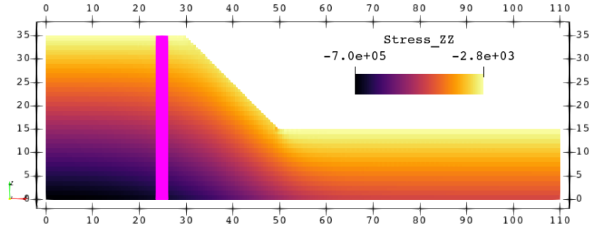
Figure 12: Elastic stress field
