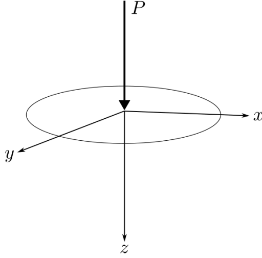
Figure 7: Boussinesq's problem.
