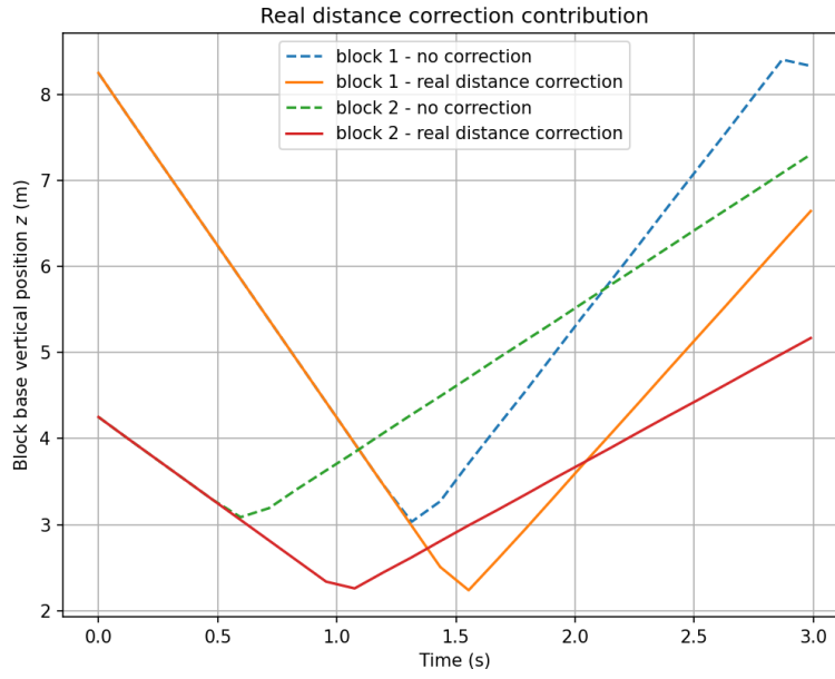
Figure 5: Displacement comparison.
