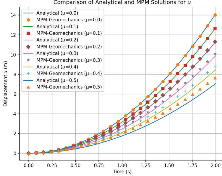
Figure 3: Verification of displacements obtained with MPM simulation.
