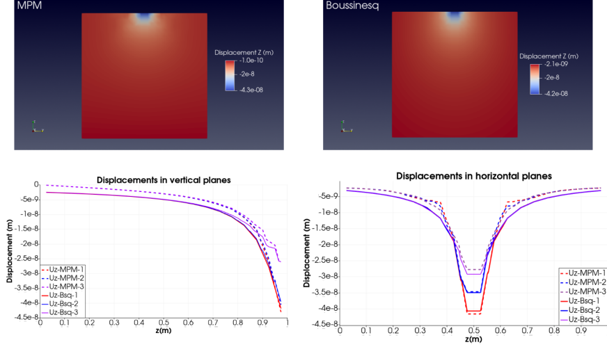
Figure 8: Comparison between analytical and MPM results.
