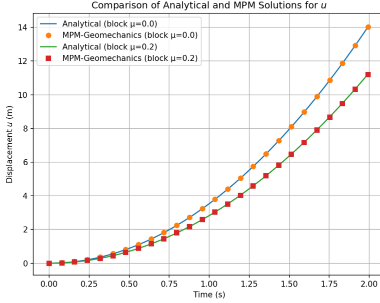
Figure 4: Verification of displacements obtained with MPM simulation.
