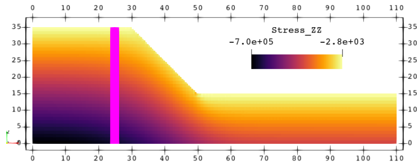
Figure 12: Elastic stress field
