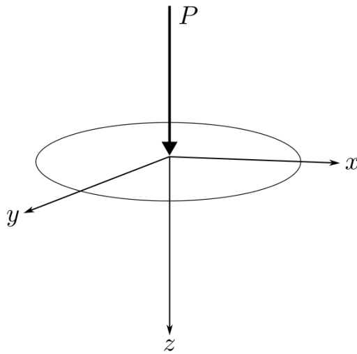
Figure 7: Boussinesq's problem.
