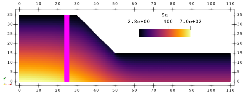
Figure 13: S_u factor obtained from initial stress field
