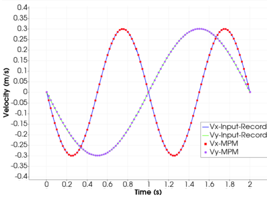
Figure 11: Verification of velocities obtained with MPM simulation.
