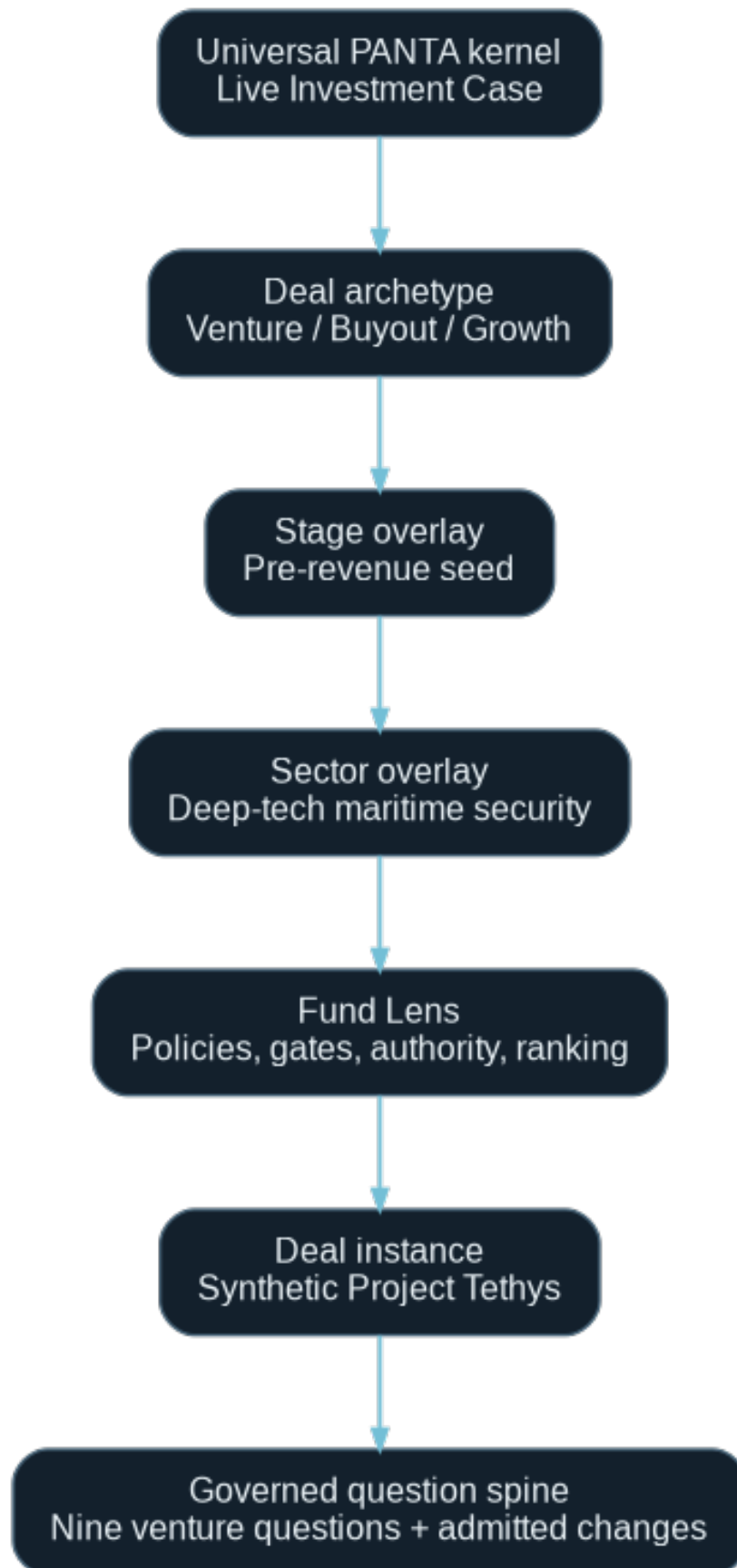
Figure 1: Archetype hierarchy
