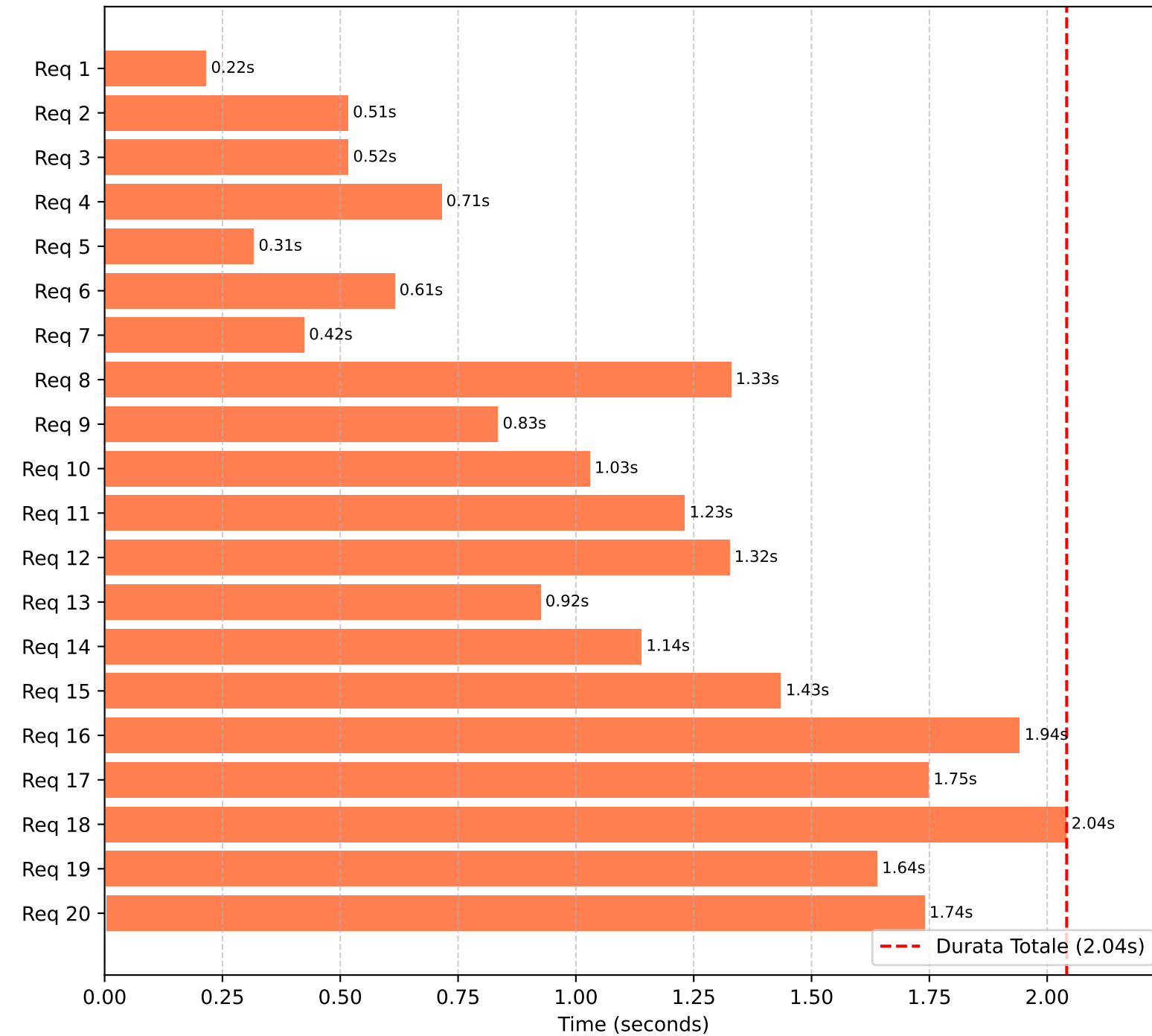
HTTP/1.1 (20 requests)
