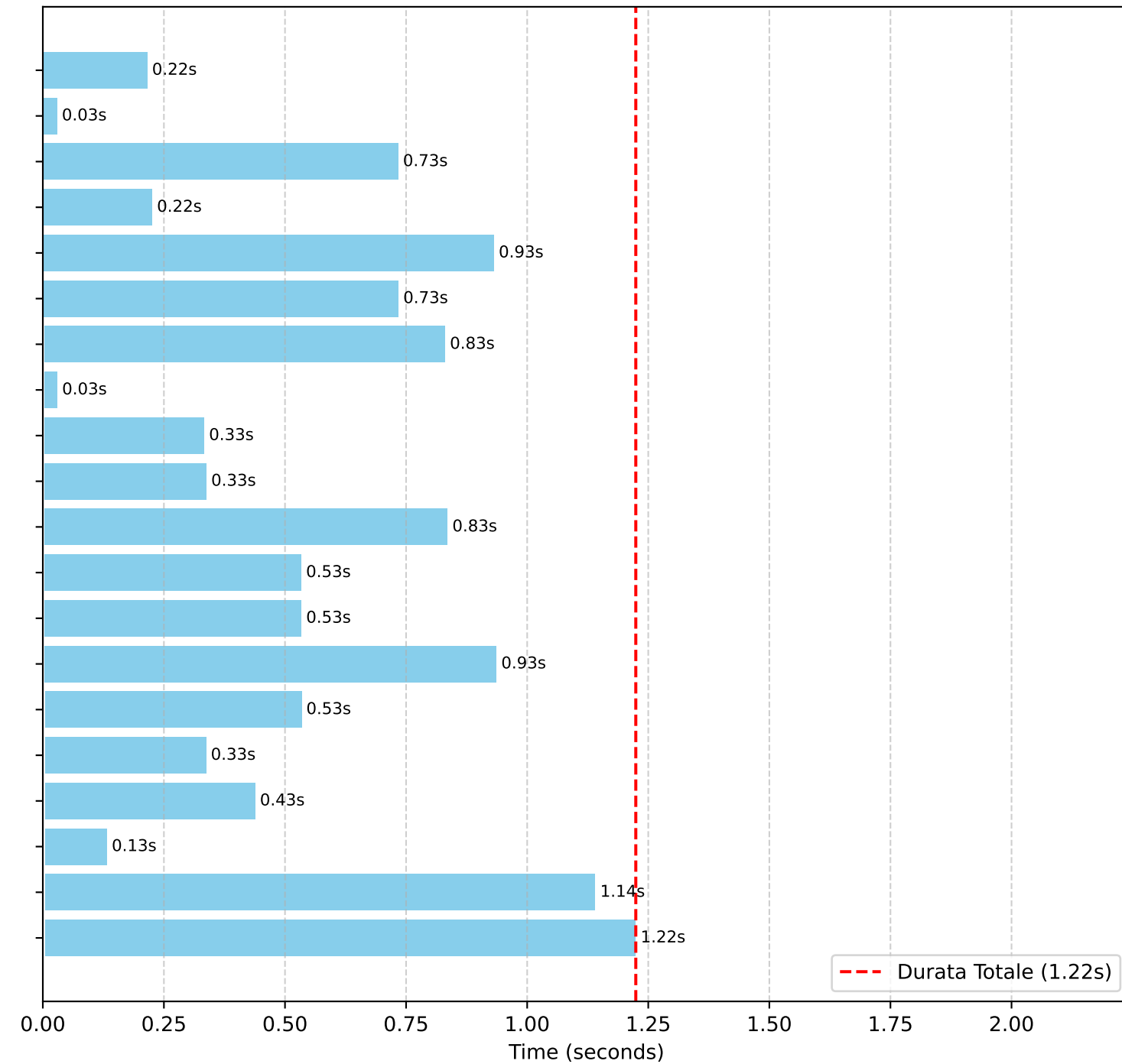
HTTP/2 (20 requests)
