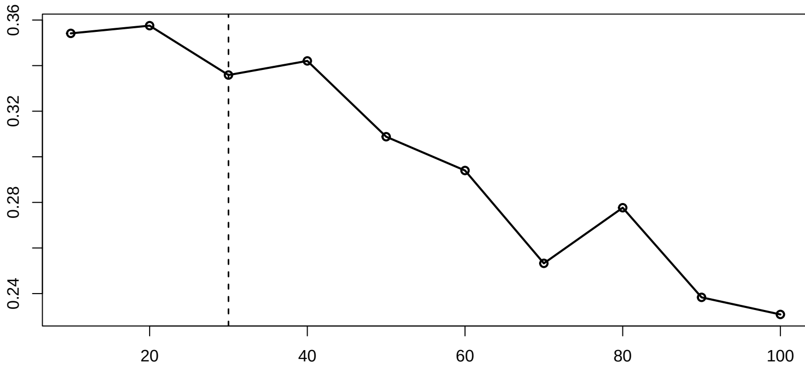
Oliveira 2015 – Sim6 (exec 1) | Kernel Radial_0.001 | F1 classe 0
