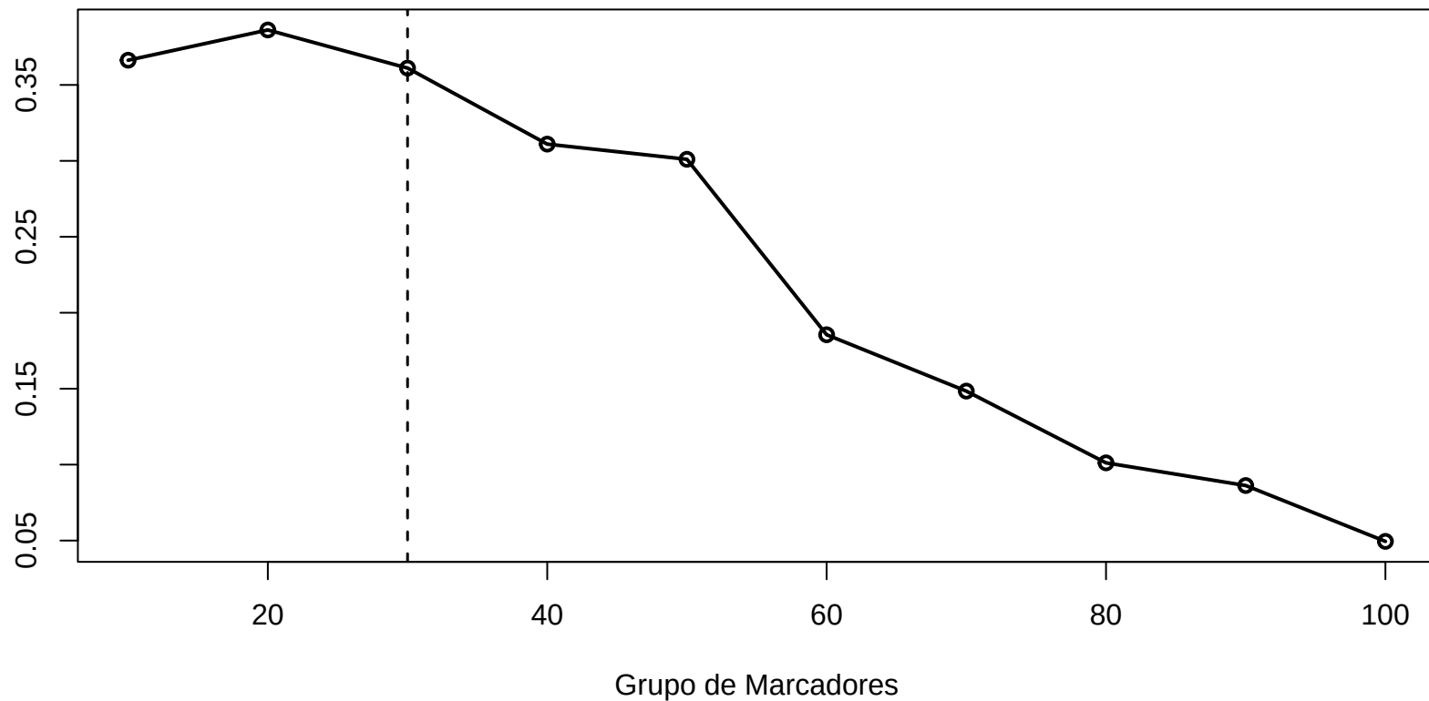
Oliveira 2015 – Sim6 (exec 1) | Kernel Radial_0.01 | F1 classe 0
