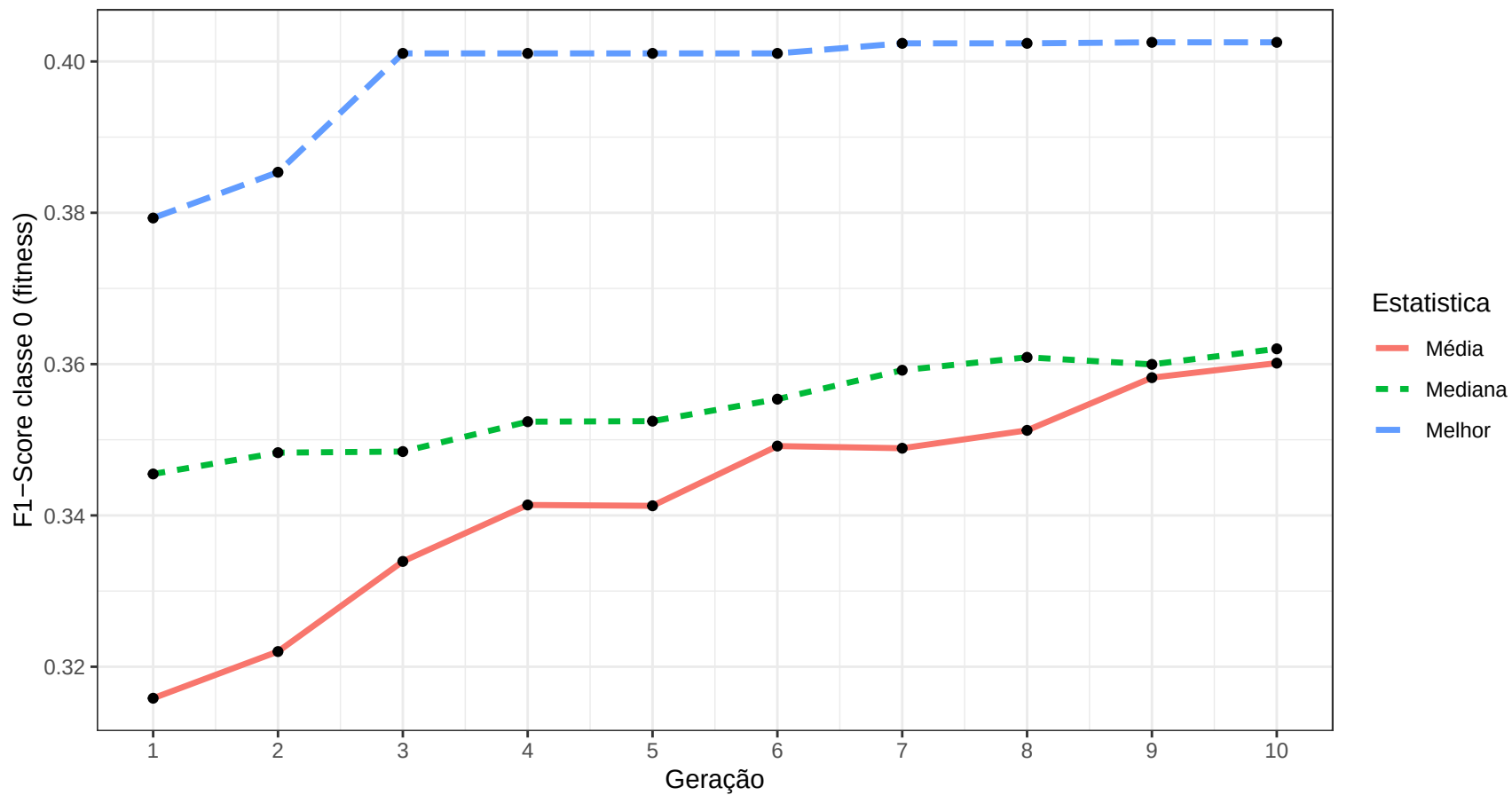
GA – F1 Minoria | Linear | Exec 1 | Oliveira 2015 Sim6
