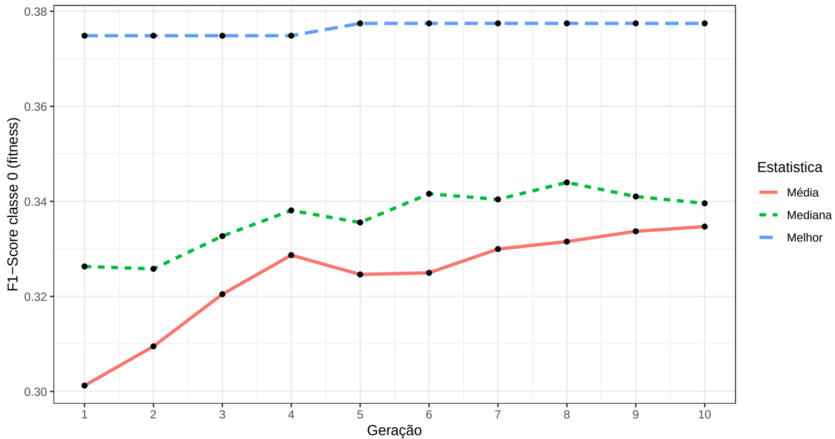
GA – F1 Minoria | Radial_0.001 | Exec 1 | Oliveira 2015 Sim6
