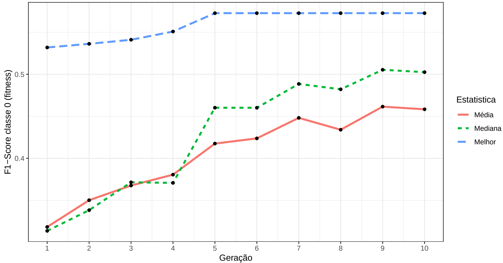
GA – F1 Minoria | Radial_0.1 | Exec 1 | Oliveira 2015 Sim6
