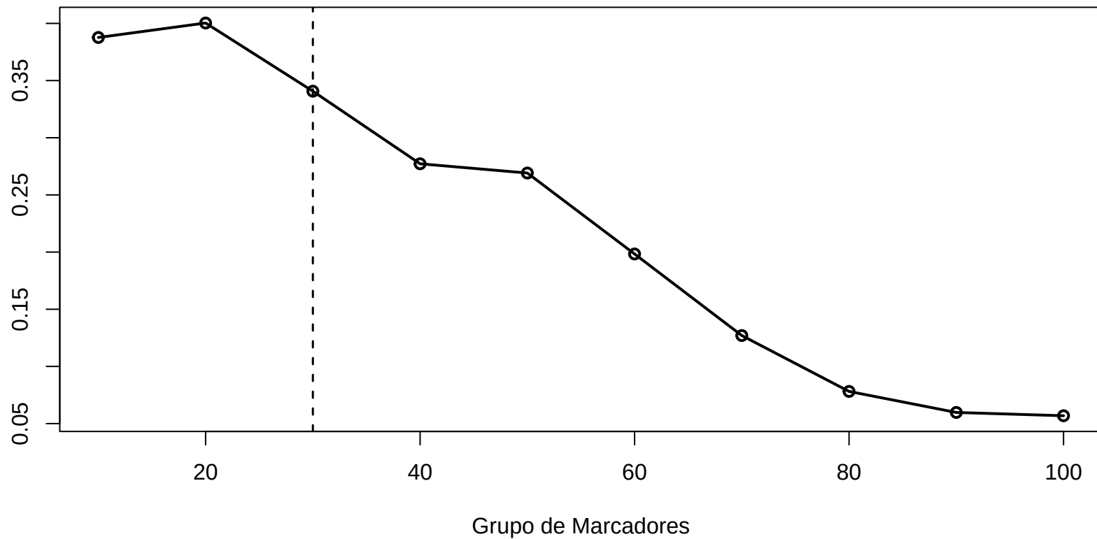
Oliveira 2015 – Sim6 (1 base, exec 1) | Kernel Radial_0.01
