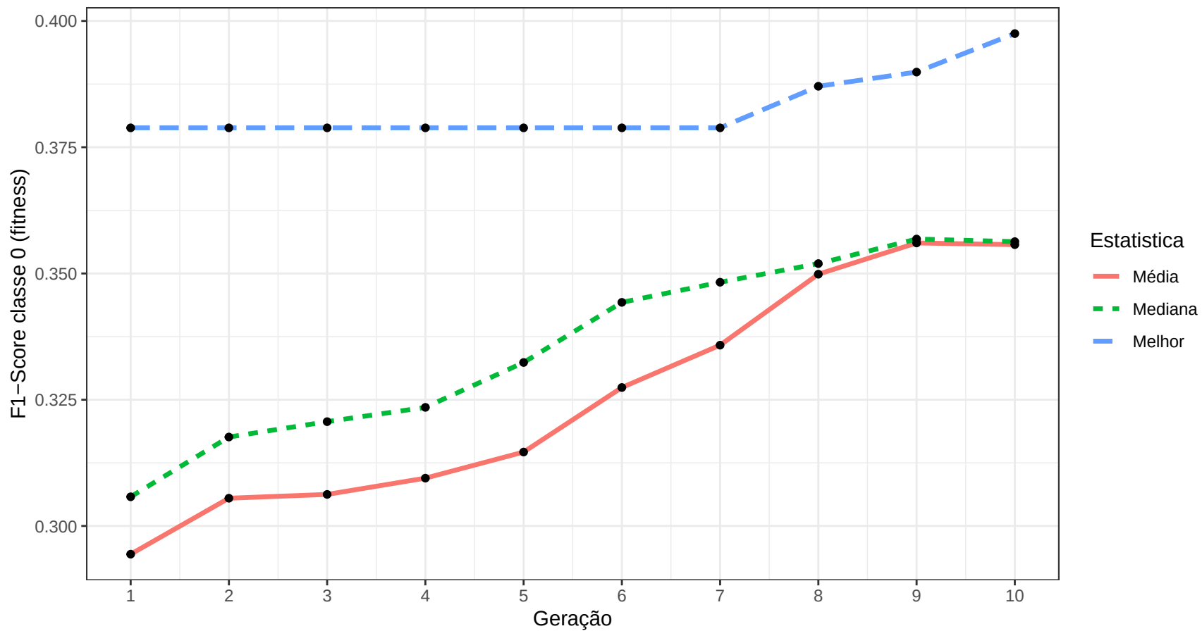
GA – F1 Minoria | Radial_0.001 | Exec 1 | 1 base × 10 exec
