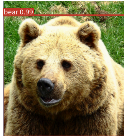
1 box (truth: 1)
