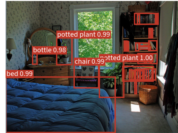
31 boxes (truth: 17)
