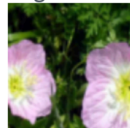
augmented
