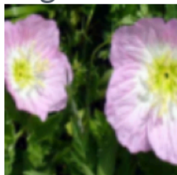
augmented
