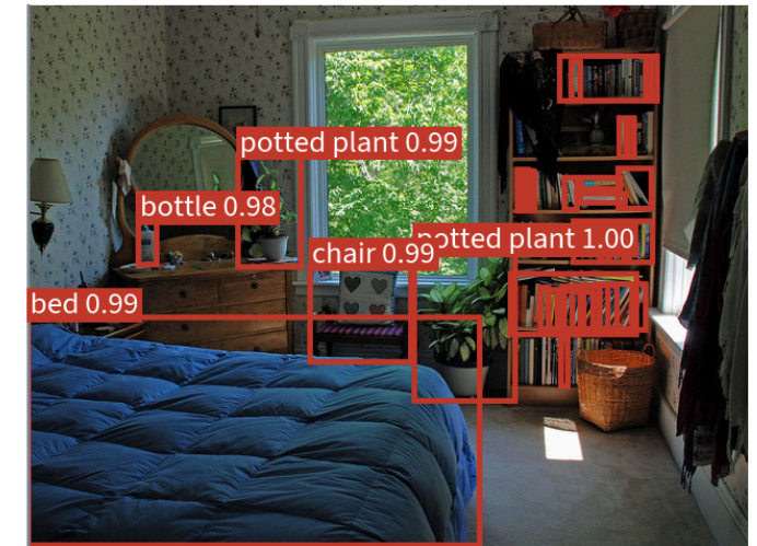
31 boxes (truth: 17)
