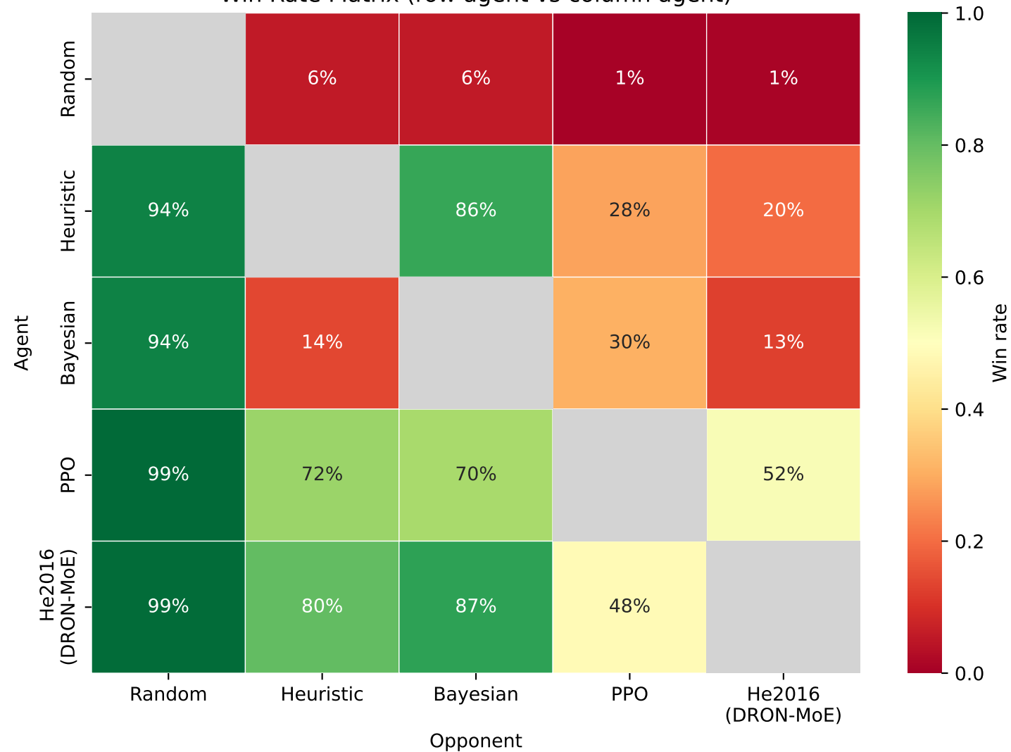
Win Rate Matrix (row agent vs column agent)
