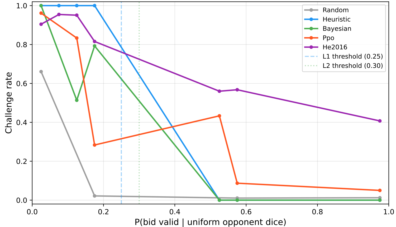
Challenge Calibration by Agent
