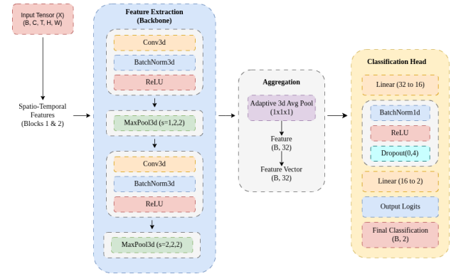
Fig. 1. Temporal CNN-based classification architecture.
