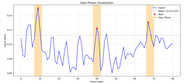
Fig. 5. Micro Expression Phase Detection Result.
