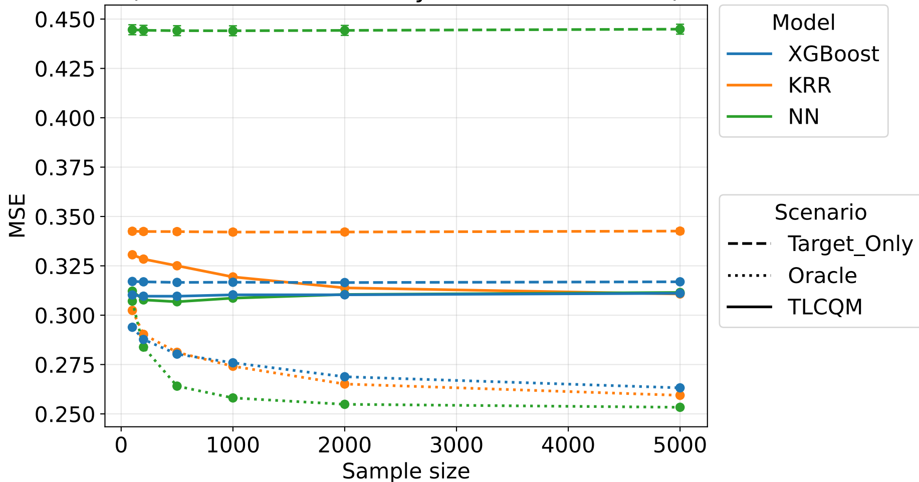
MSE vs Sample Size (Color = Model, Linestyle = Data Scenario)
