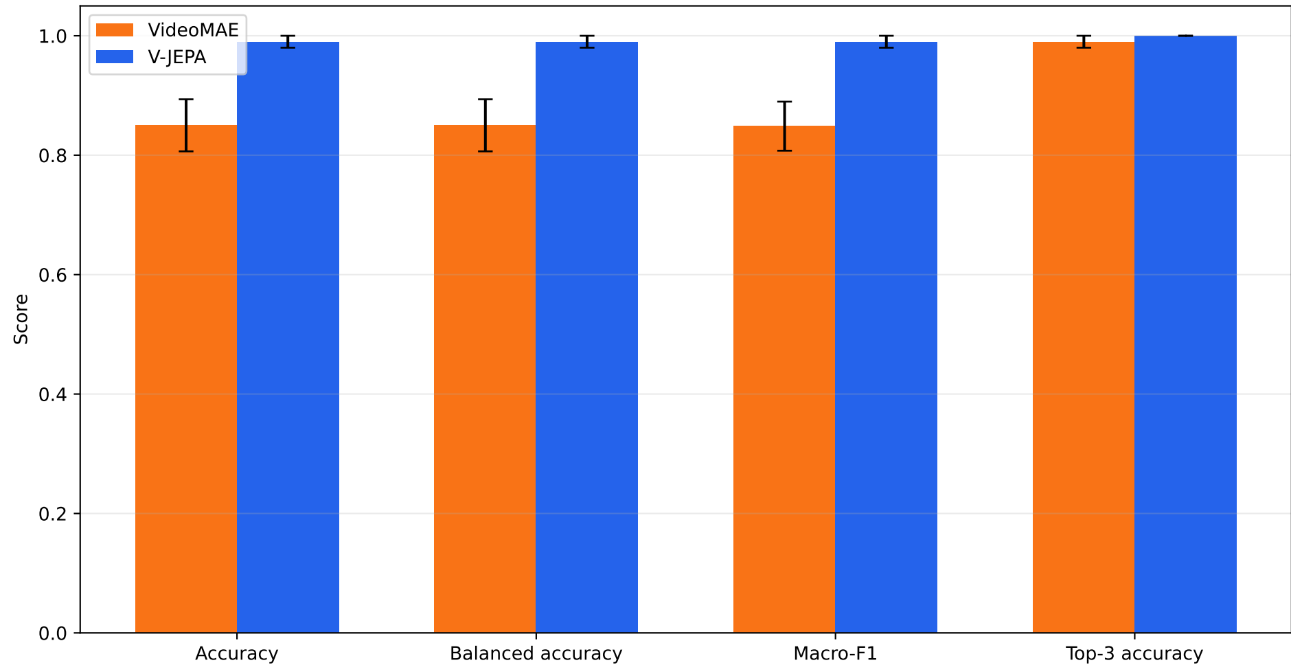
Frozen-feature linear probe on UCF101 (mean \pm std, 3 splits)
