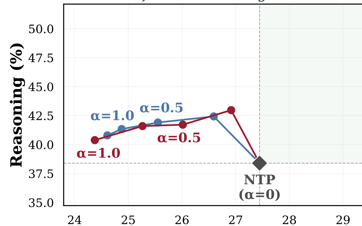
Post-training after mid-training KD
