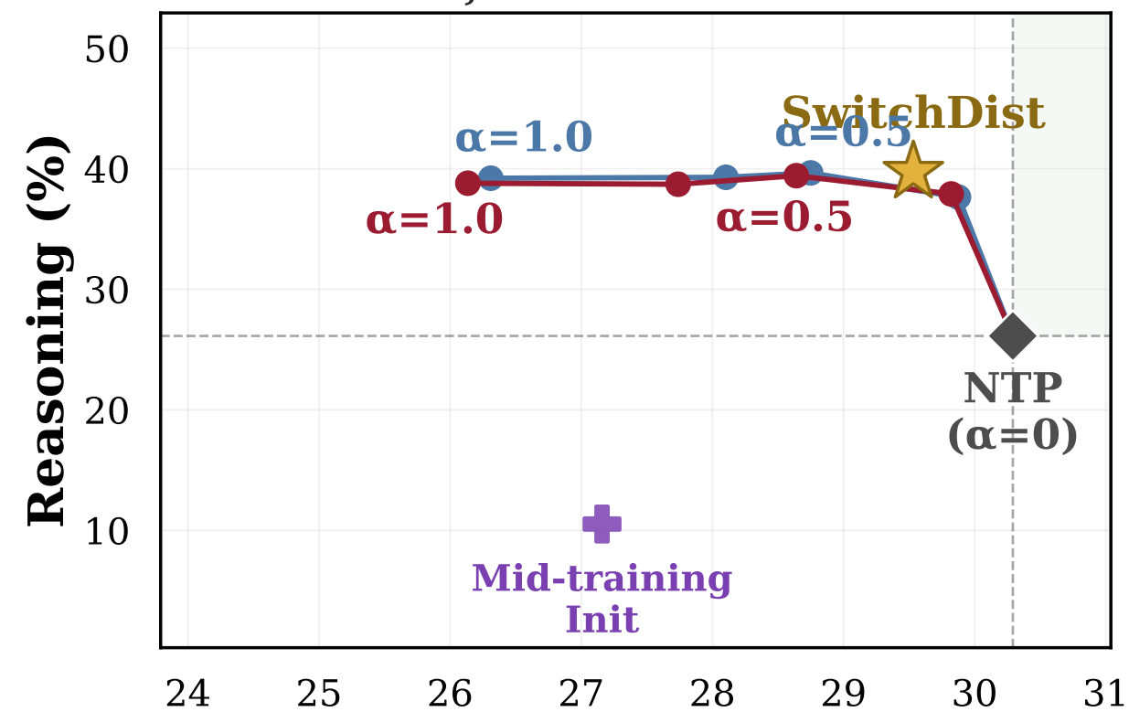
Mid-training after 60B tokens
