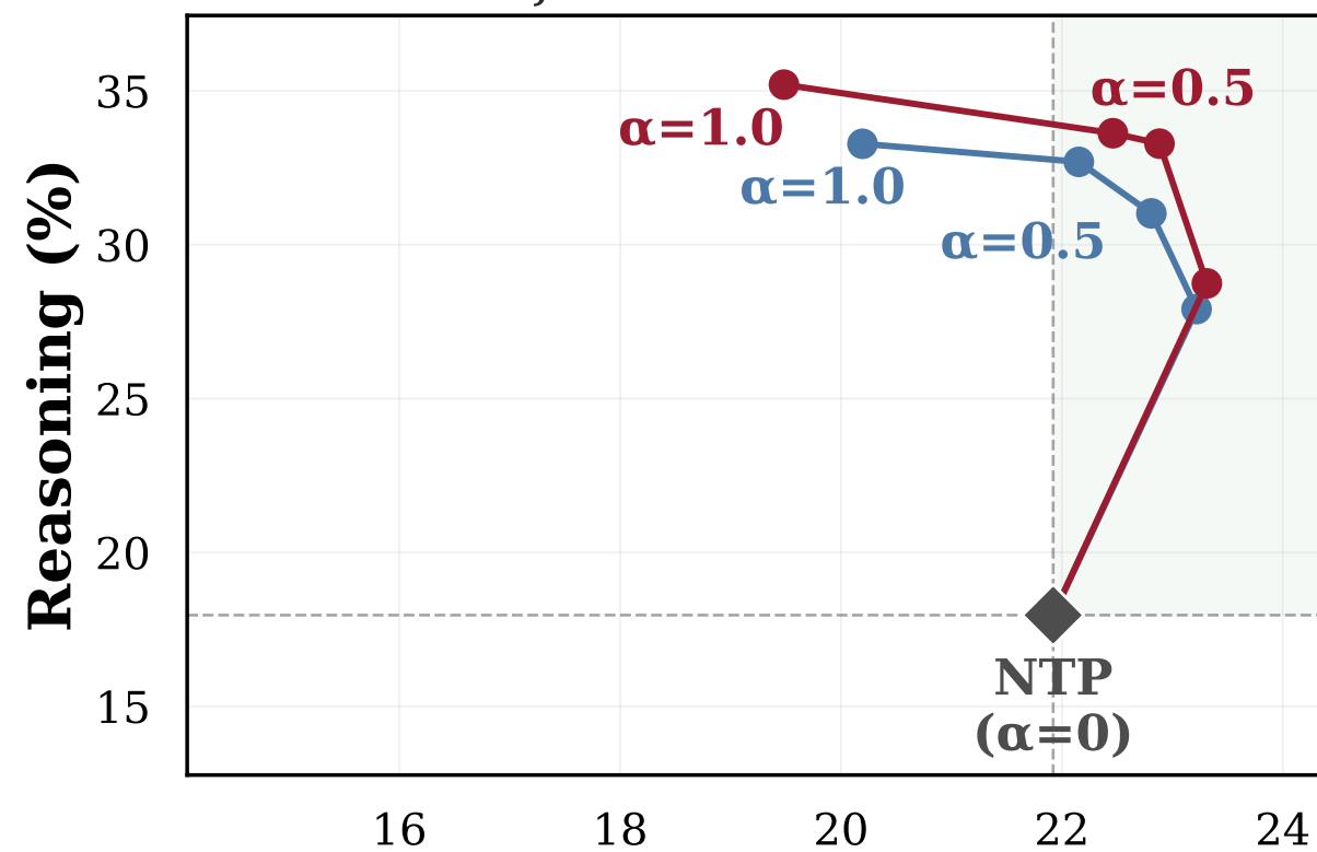
Pre-training after 100B tokens
