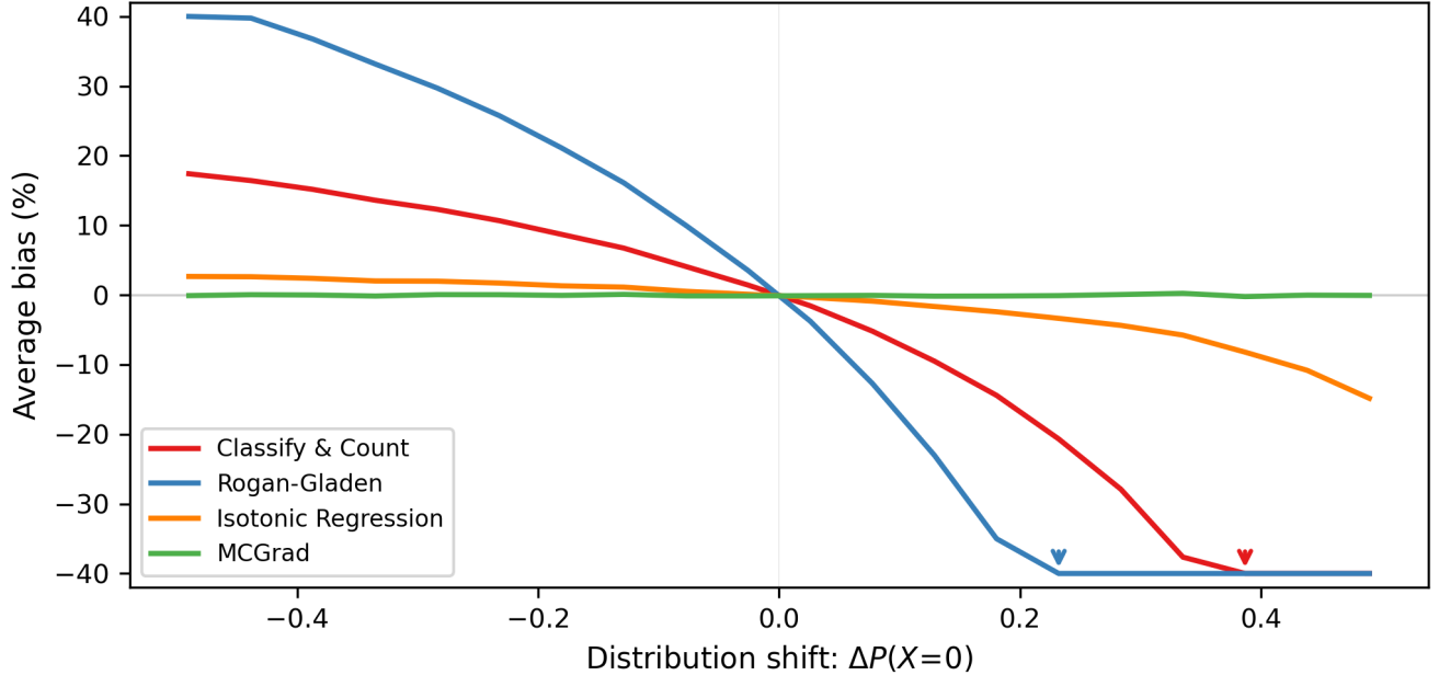
Figure 1: Prevalence estimation bias (% relative) under covariate shift, averaged over 50 simulation runs. The x -axis shows \Delta P(X=0) , the change in P(X=0) from the training value of 0.5. Classify & Count and Rogan-Gladen diverge with increasing shift (arrows indicate values beyond the axis range); isotonic regression (global calibration) shows moderate bias; MCGrad maintains near-zero bias across all shift levels. Additional methods (PACC, SLD, uncalibrated) shown in SI Appendix Figure S2.
