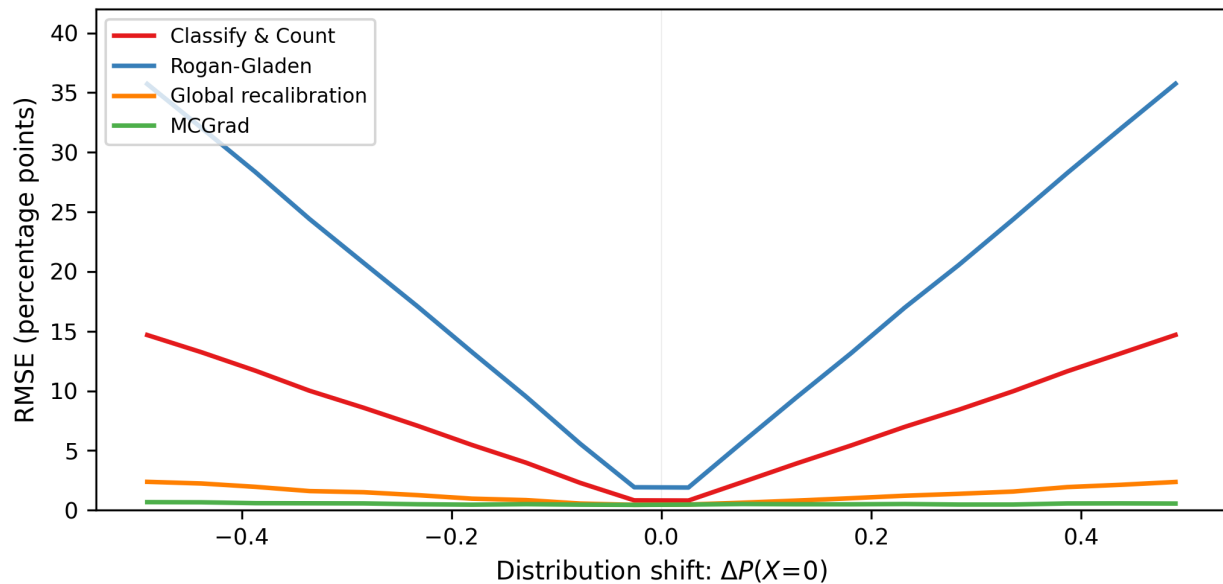
Figure S1: Root mean squared error (RMSE) under covariate shift for the four methods in main-text Figure 1 (Classify & Count, Rogan-Gladen, multiplicative global recalibration, MCGrad), averaged over 50 simulation runs. RMSE closely tracks absolute bias for all methods, confirming that variance is small relative to bias at this sample size. MCGrad maintains the lowest RMSE across all shift levels.
