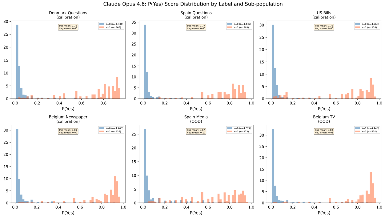
Figure S4: Claude Opus 4.6 P(\text{Yes}) score distribution by label across six CAP sub-populations. Scores are well-separated (mean 0.75 for positives vs. 0.07 for negatives) with 43 unique values and no boundary mass.
