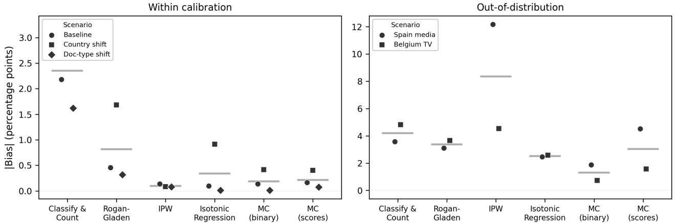
Figure 3: Prevalence estimation |\text{bias}| (percentage points) across the shift gradient. Each marker shape represents a different shift scenario; horizontal lines show the mean across scenarios. MCGrad achieves near-zero bias within the calibration distribution in both binary-label and probability-score conditions. Full numerical results in SI Appendix Table S2.
