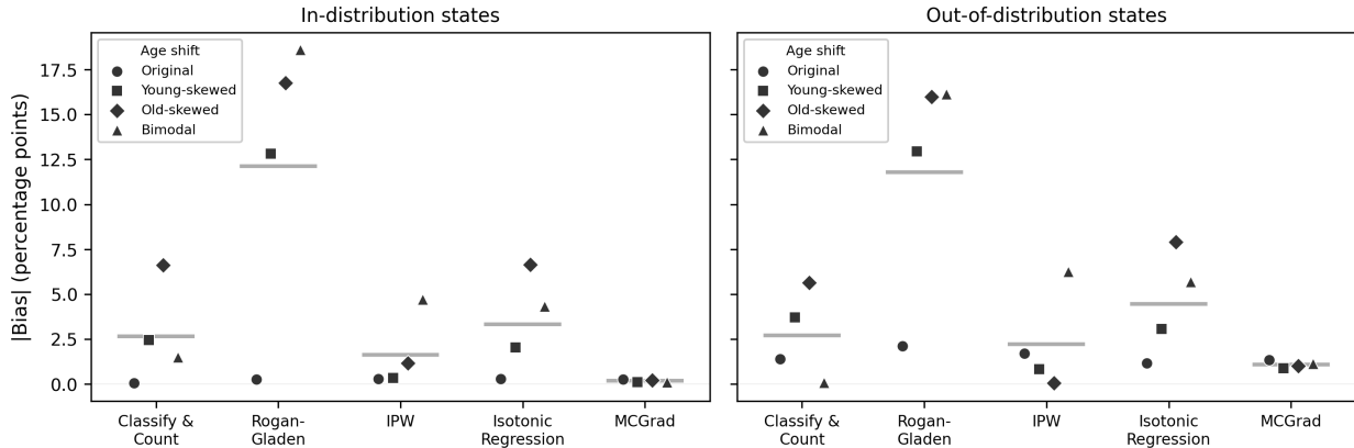
Figure S5. Absolute prevalence bias (percentage points) for the ACS employment benchmark, by method and age-shift scenario, for in-distribution (left) and out-of-distribution (right) states. Marker shape denotes the synthetic age distribution; horizontal lines are per-method means. MCGrad is near-unbiased across all in-distribution scenarios (including the bimodal shift that defeats IPW) and degrades only modestly out of distribution; Rogan-Gladen and isotonic regression grow with the age shift.
