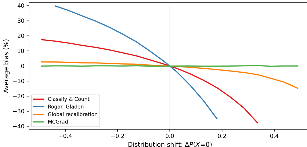
Figure S4. Relative prevalence bias under covariate shift (50 runs). The x-axis is the change in P(X = 0) from the training value of 0.5. Classify & Count and Rogan-Gladen diverge with shift; global recalibration (multiplicative, the method of Section S1.6) shows moderate bias; the multicalibrated estimator stays near zero. Cropped at \pm 40\% ; see Figure S2 for the full range and additional methods.
