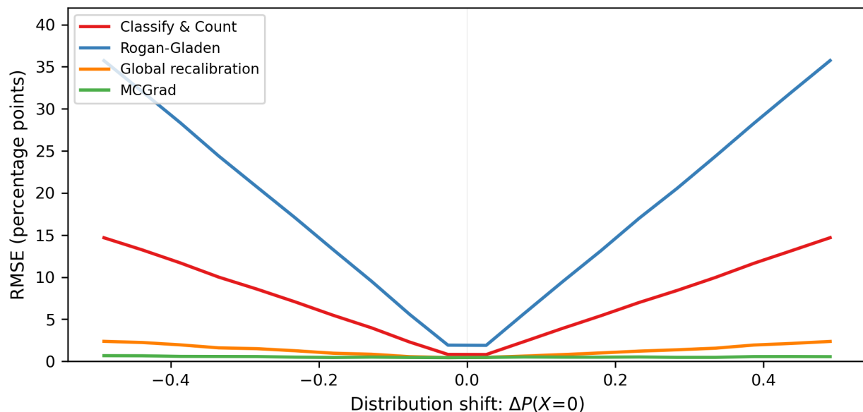
Figure S1: Root mean squared error (RMSE) under covariate shift for the same four methods shown in Figure S4 (Classify & Count, Rogan-Gladen, multiplicative global recalibration, MCGrad), averaged over 50 simulation runs. RMSE closely tracks absolute bias for all methods, confirming that variance is small relative to bias at this sample size. MCGrad maintains the lowest RMSE across all shift levels.
