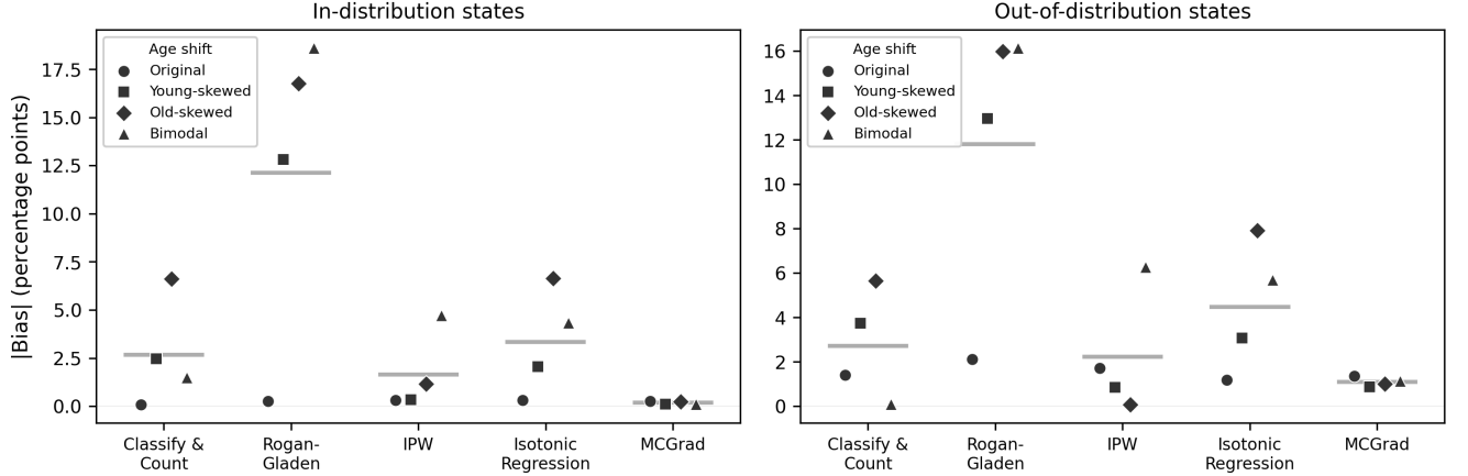
Figure 2: Prevalence estimation |bias| (percentage points) under synthetic age distribution shift, for in-distribution states (left) and out-of-distribution states (right). Each marker shape represents a different age shift scenario; horizontal lines show the mean across scenarios. Full numerical results in SI Appendix Table S1.
