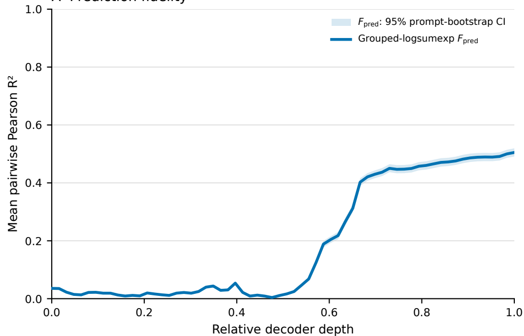
A Prediction fidelity
