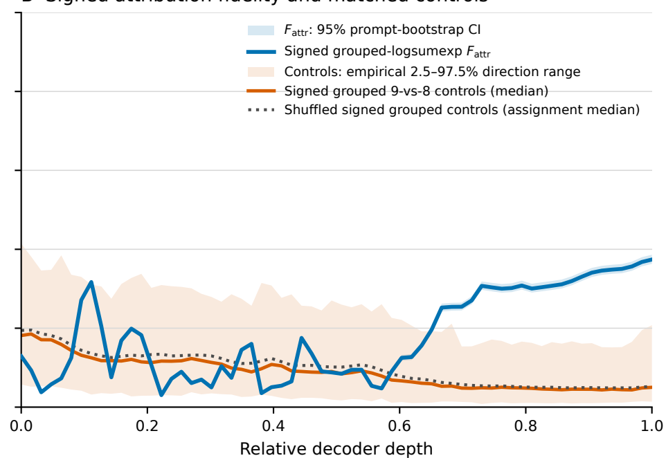
B Signed attribution fidelity and matched controls
