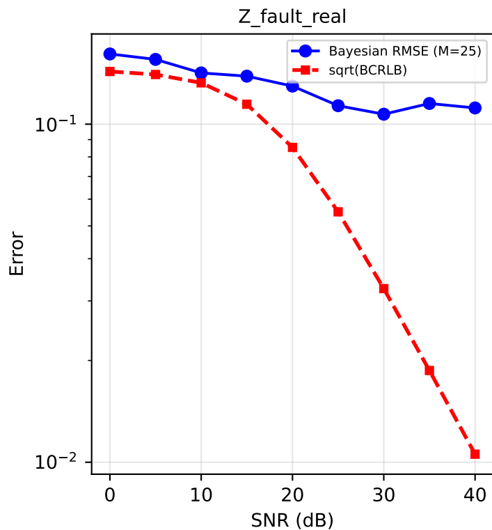
Bayesian RMSE vs sqrt(BCRLB) - SNR Sweep ( \alpha=5.0 , M=25 trials per SNR)
