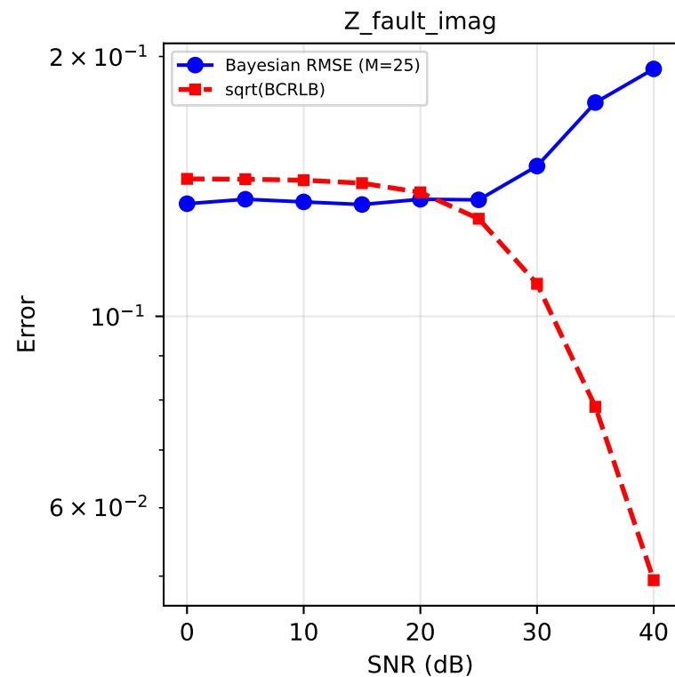
Bayesian RMSE vs sqrt(BCRLB) - SNR Sweep ( \alpha=5.0 , M=25 trials per SNR)
