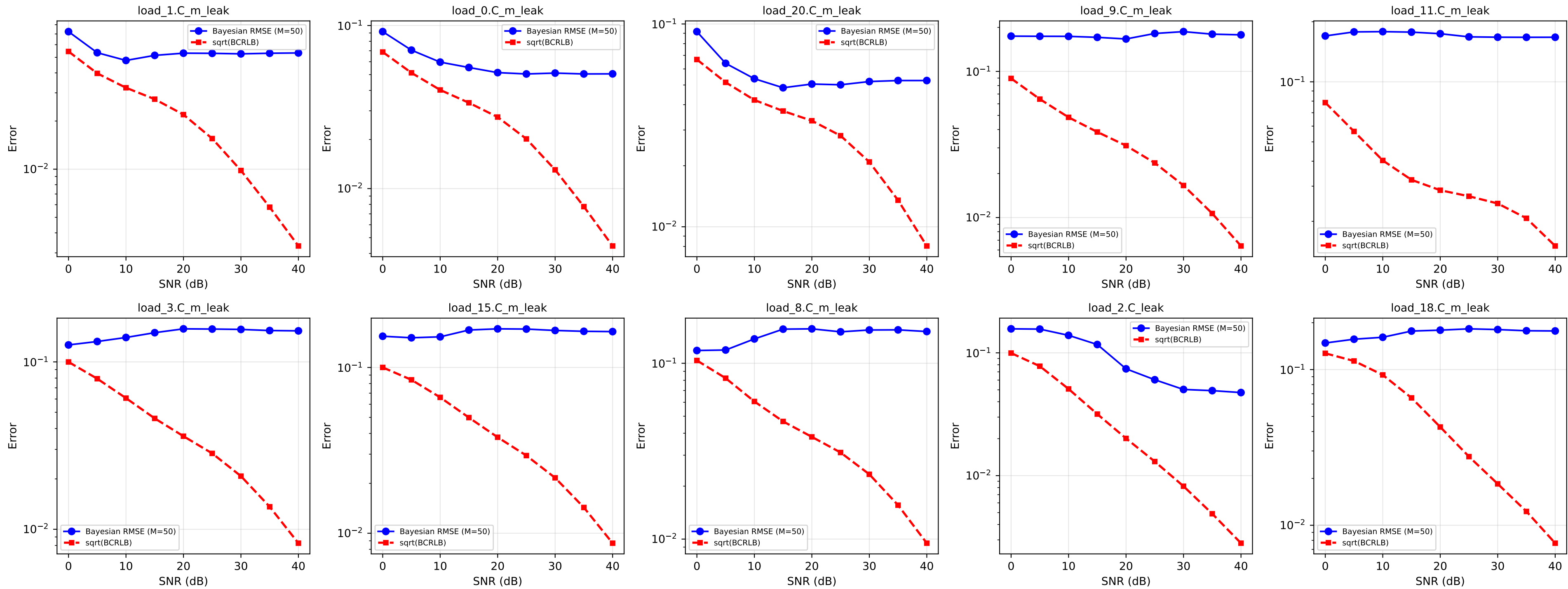
Bayesian RMSE vs sqrt(BCRLB) - SNR Sweep ( \alpha=5.0 , M=50 trials per SNR)
