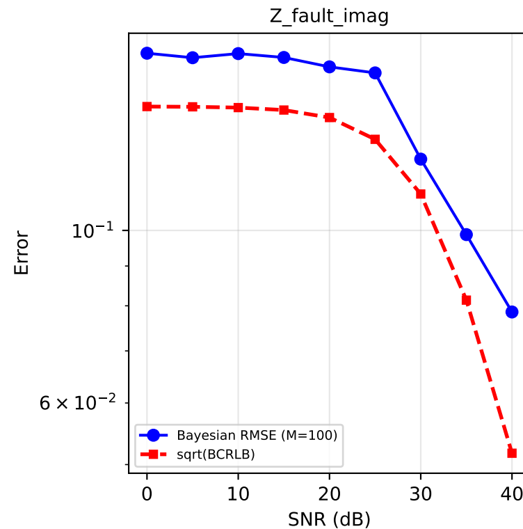
Bayesian RMSE vs sqrt(BCRLB) - SNR Sweep ( \alpha=5.0 , M=100 trials per SNR)
