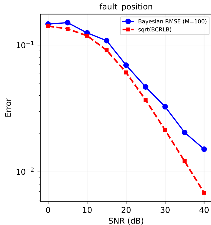
Bayesian RMSE vs sqrt(BCRLB) - SNR Sweep ( \alpha=5.0 , M=100 trials per SNR)
