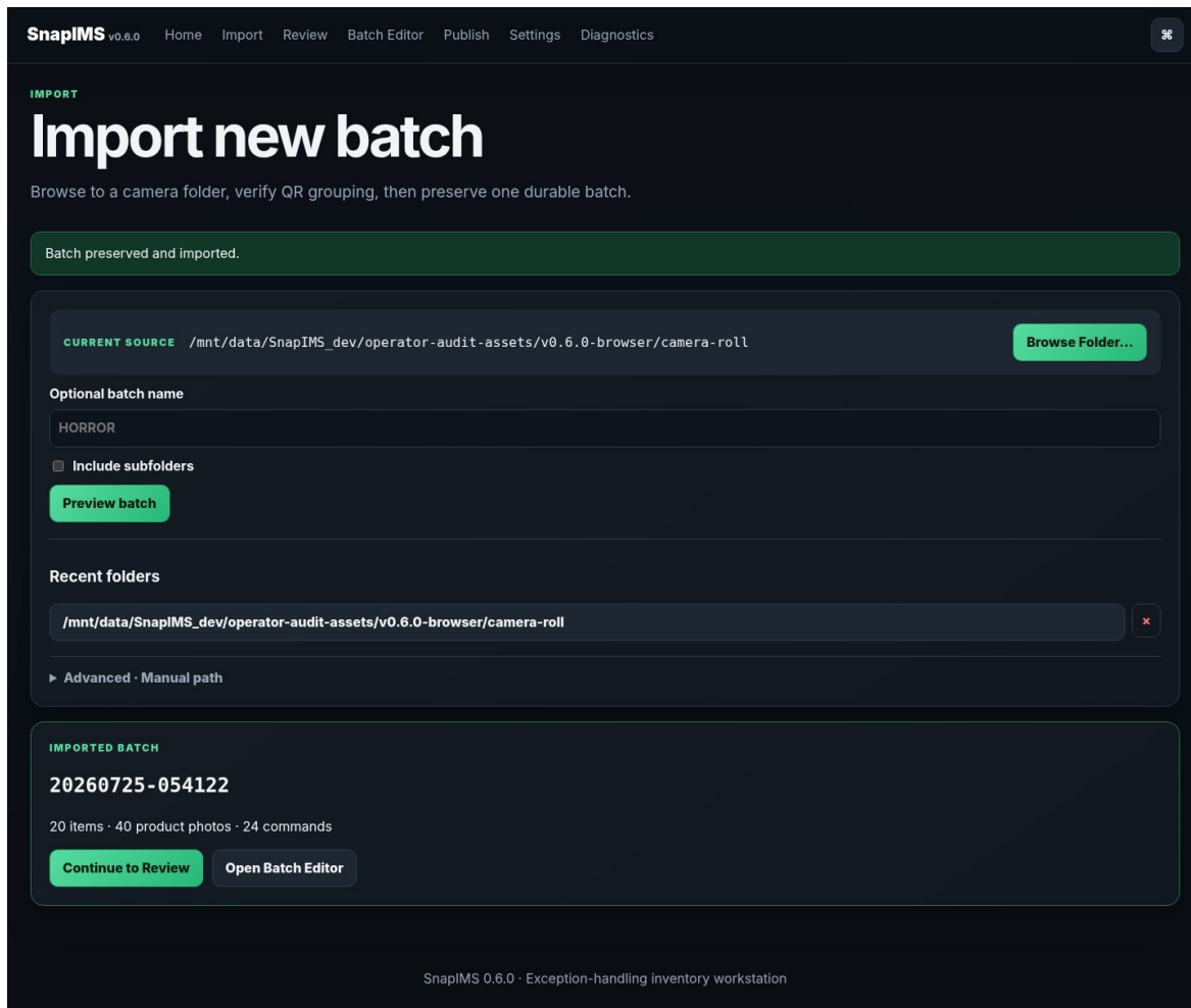
Durable batch created after preservation
