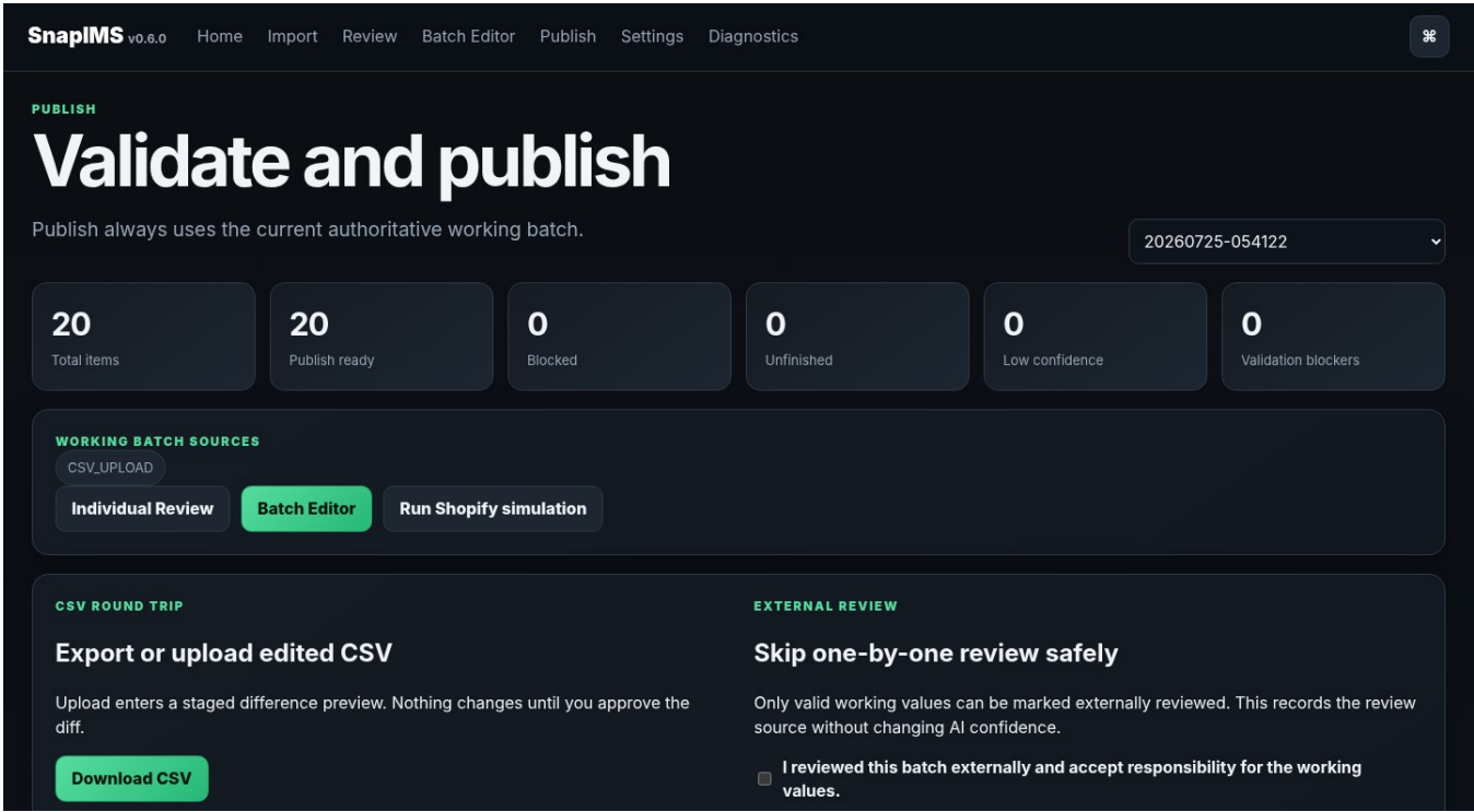
Publish validation and Shopify simulation - view 1 of 4
