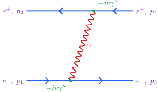
(b) t -channel exchange: q^2 = t
