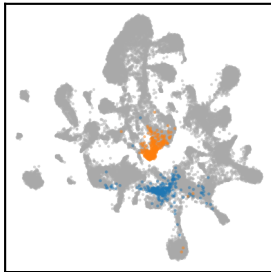
SATURN-ArcFace
