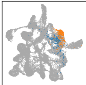
SATURN-triplet
