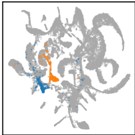
GECross
