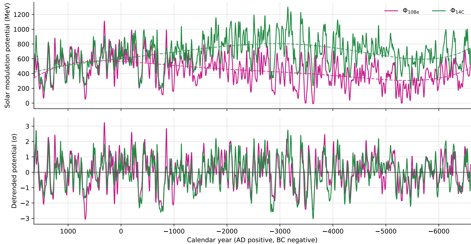
Solar modulation potential and degree-5 long-term trends
