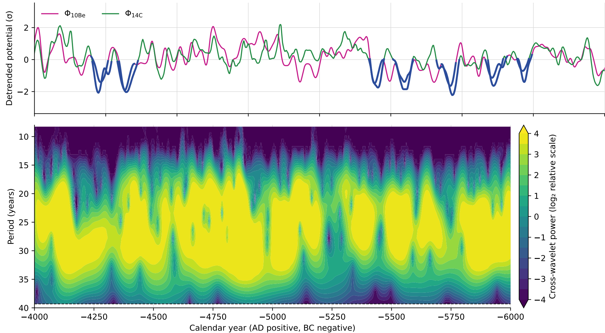
Cross-wavelet behavior during selected grand minima
