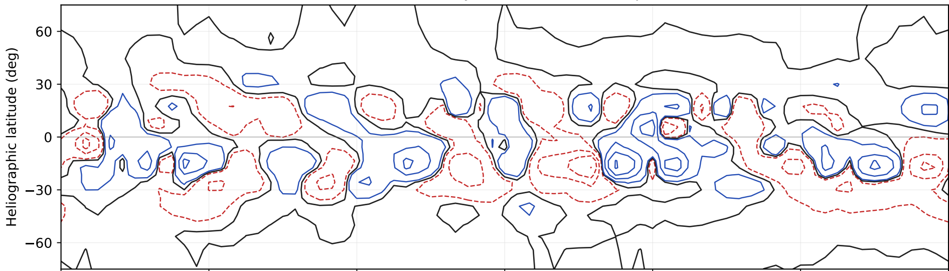
(b) CR 1917: Solar-cycle 23 minimum - December 1996
