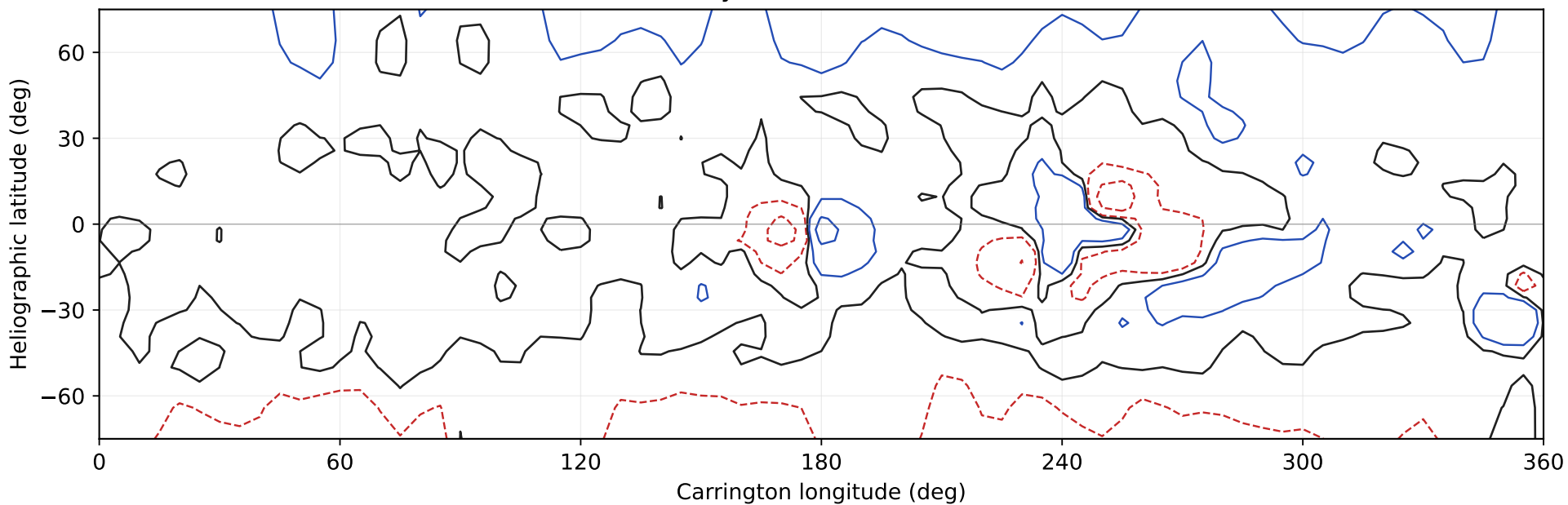
(b) CR 1917: Solar-cycle 23 minimum - December 1996
