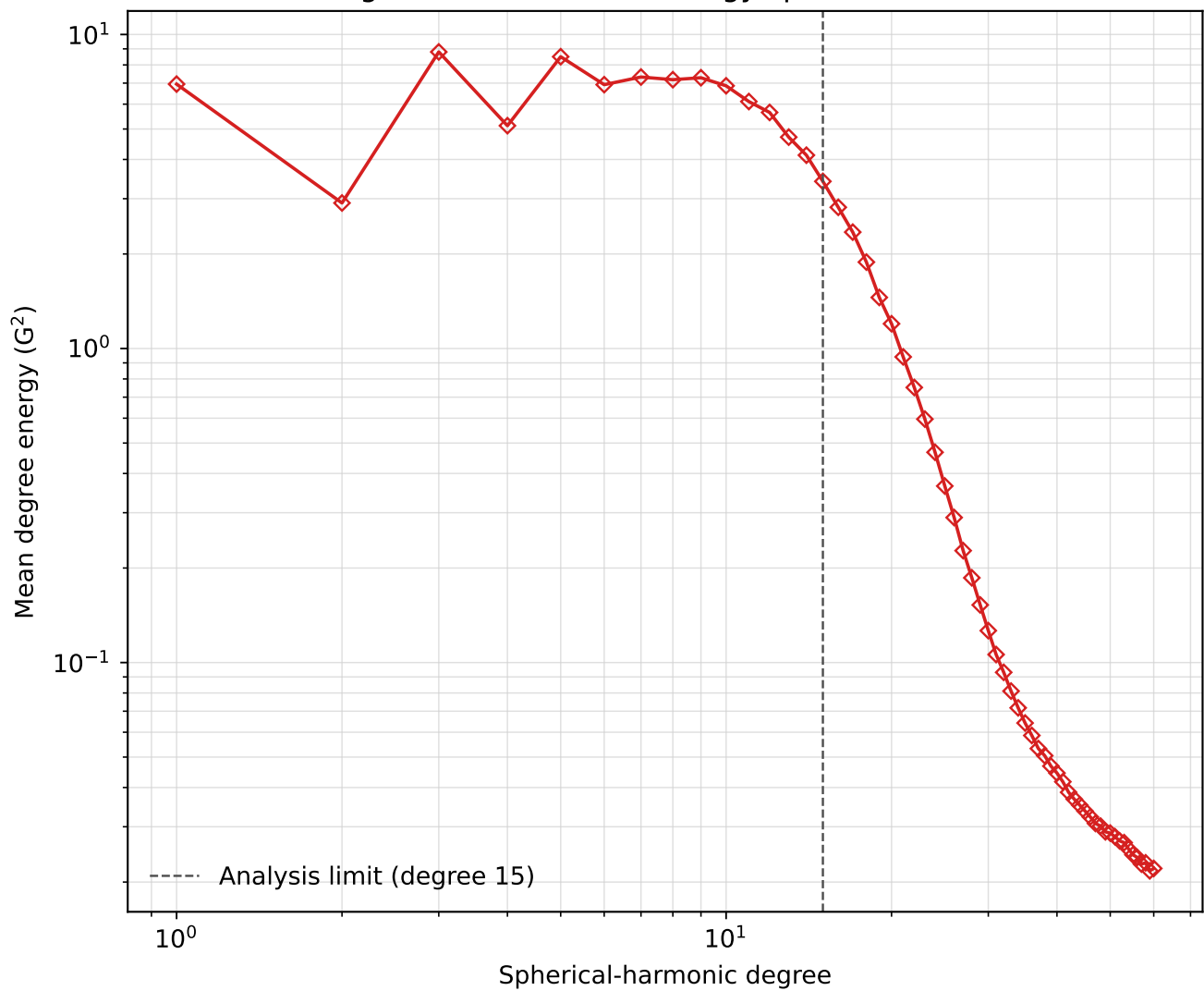
Time-averaged WSO harmonic-energy spectrum, CR 1642-2182
