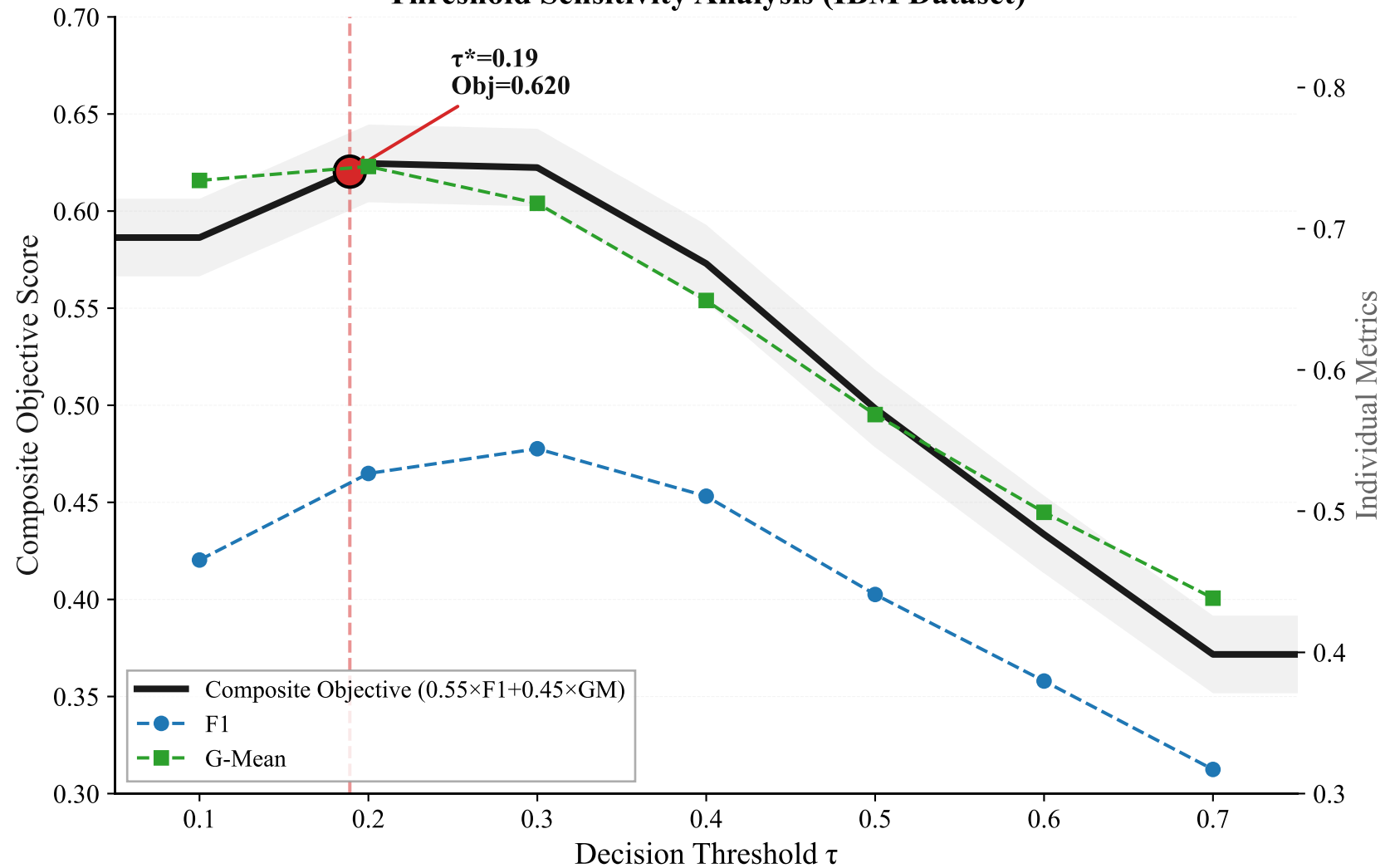
Threshold Sensitivity Analysis (IBM Dataset)
