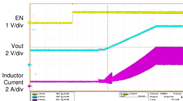
Figure 8-5. Startup Waveforms
