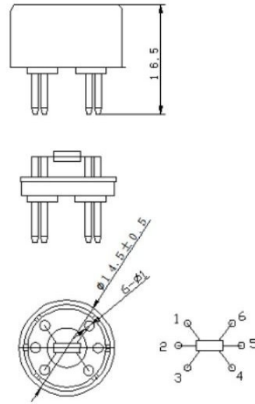
Fig1. Sensor Structure
